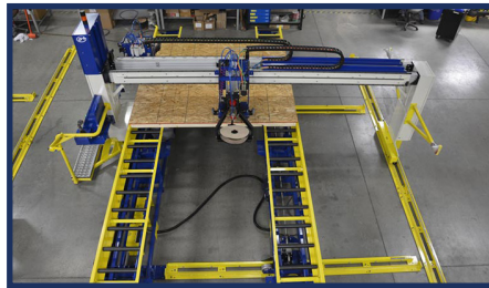
Dual Beam Sheathing Station
