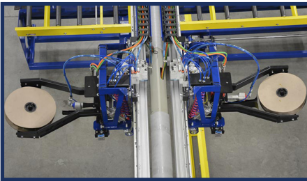
Dual Beam Bridge
