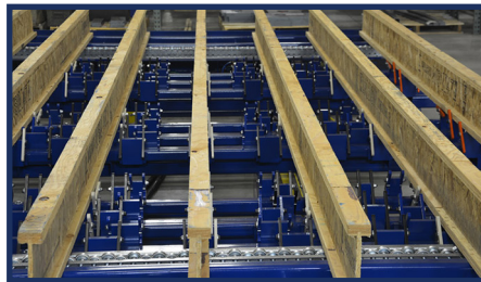
Joists Placed on Table
