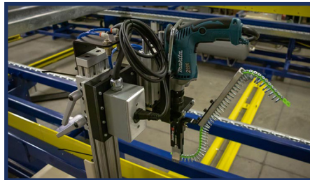
Screw Tool Carriage *Tool not included
