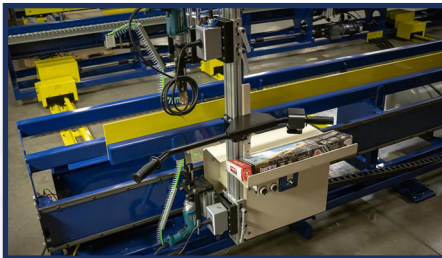
Framing Table with Screw Tool Carriage
